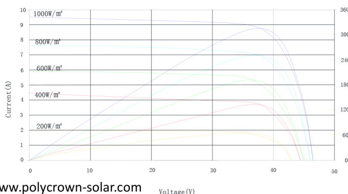
Current-Voltage&Power-Voltage Curve
